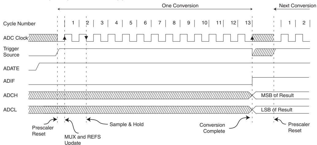
Figure 20-6. ADC Timing Diagram, Auto Triggered Conversion
