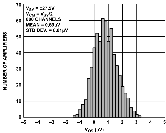
Figure 8. Input Offset Voltage Distribution, V_{SY} = \pm 27.5\text{ V}
