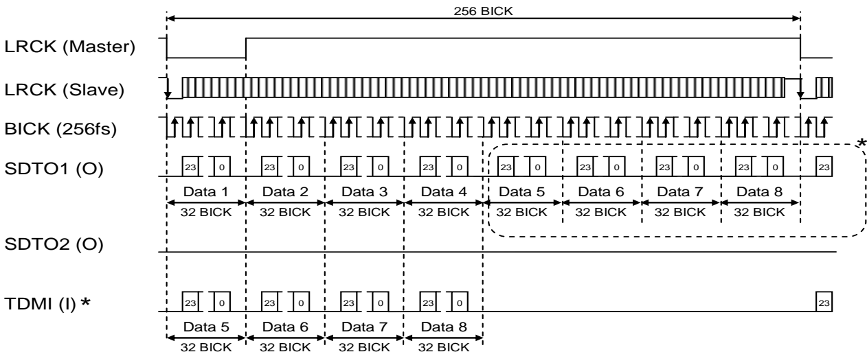
Figure 17. Model 1 Timing (TDM256 Mode (I 2 S))
