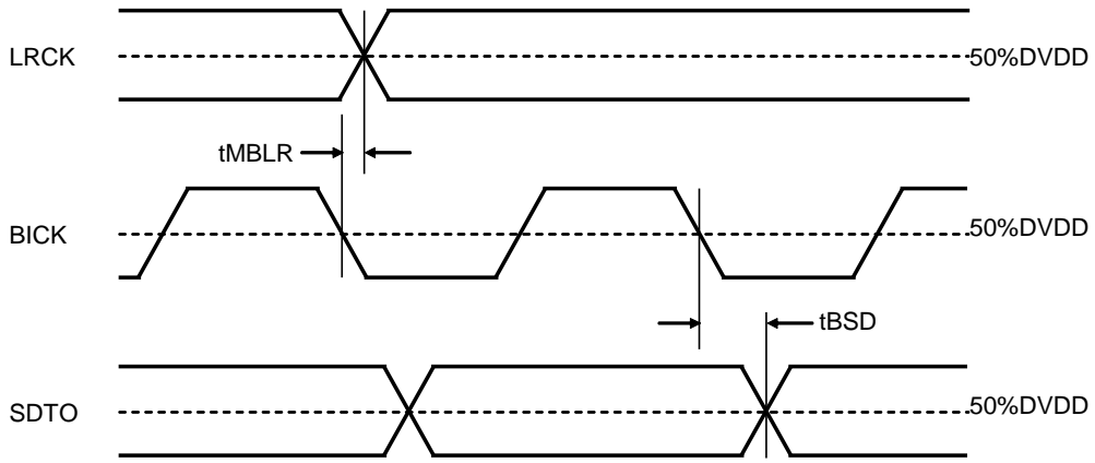
Figure 8. Audio Interface Timing (TDM1/0 bits = "00" & Master mode)
