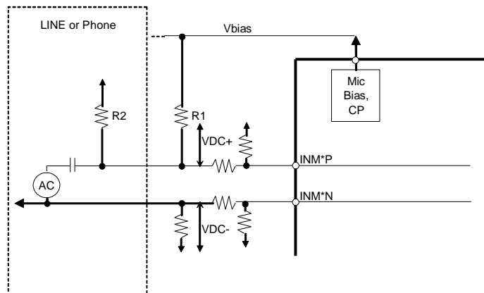
Figure 25. LINE and Phone Input Mode (IN*MP/N pins)
