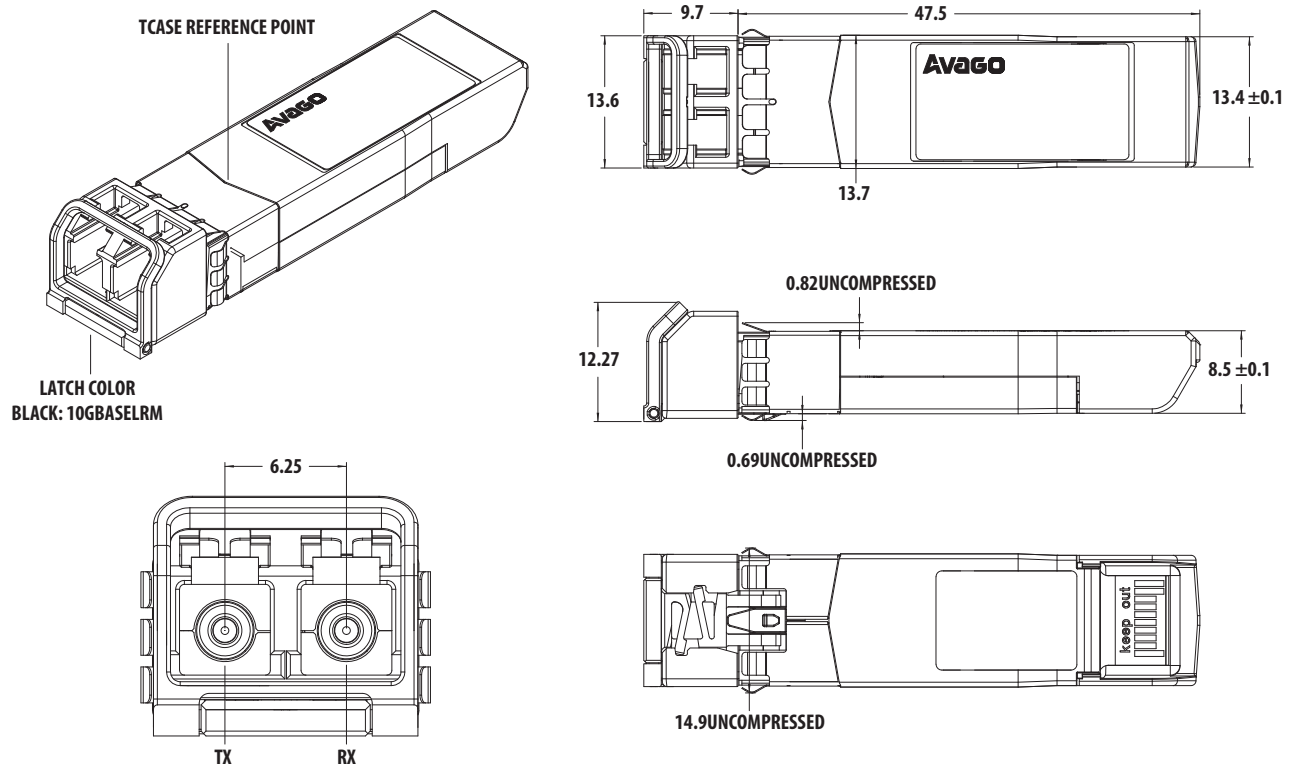
Figure 7. Module drawing
