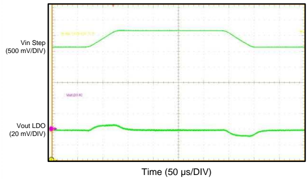
Figure 8. Buck Line Transient PWM
