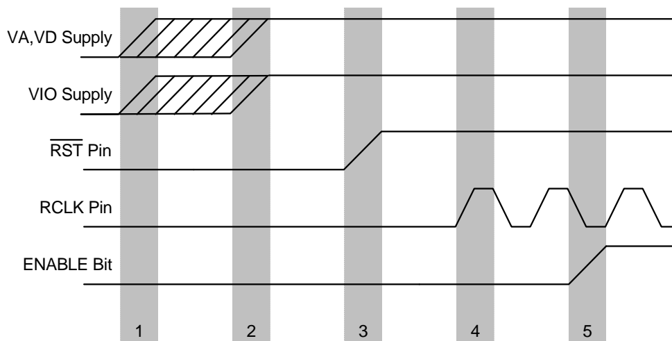
Figure 1. Initialization Sequence
