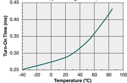
Typical Turn-On Time vs. Temperature ( I_F=5\text{mA} , I_L=80\text{mA} )
