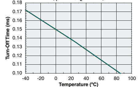
Typical Turn-Off Time vs. Temperature ( I_F=5\text{mA} , I_L=80\text{mA} )
