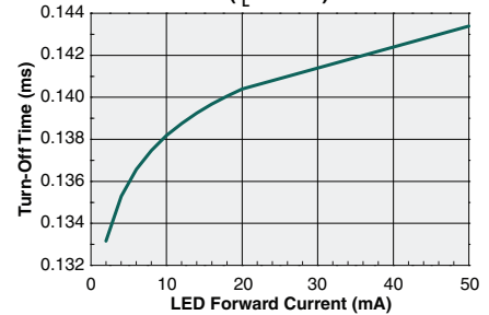
Typical Turn-Off Time vs. LED Forward Current ( I_L=30\text{mA} )
