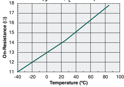
Typical On-Resistance vs. Temperature ( I_F=5\text{mA} , I_L=100\text{mA} )
